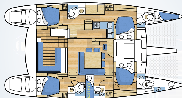
LAGOON 500 Layout
